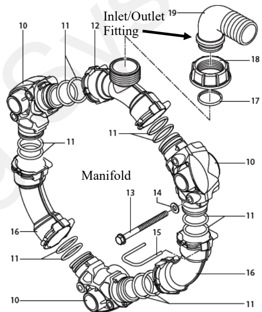
Typical Manifold—2 per pump— inlet and outlet
