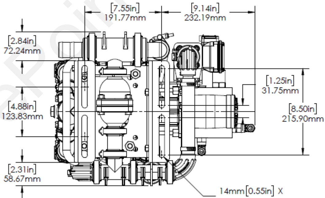
Bottom View
