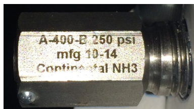
153-A-400-B 1/4" Hydrostat Relief Valve—250 PSI — (Keep the dust cap on) Used in various segments of the system as a safety relief valve.
